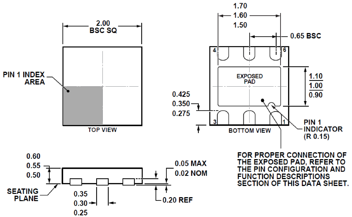
6-Lead Lead Frame Chip Scale Package [LFCSP_UD] 2.00 mm × 2.00 mm Body, Ultra Thin, Dual Lead Dimensions show in millimeters
