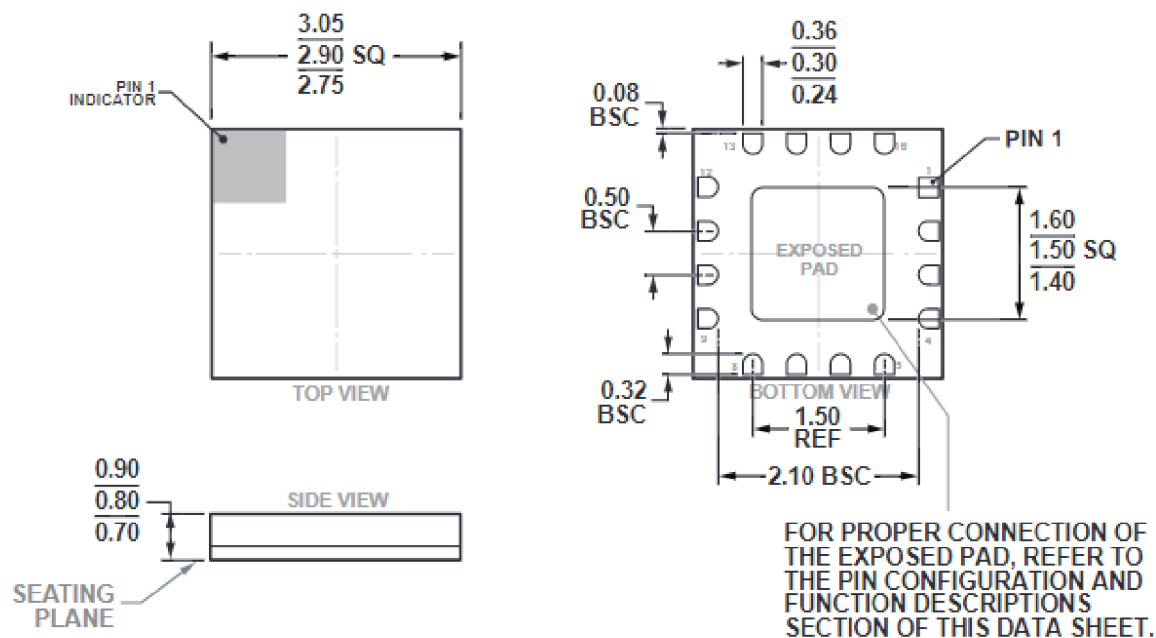
16-Terminal Ceramic Leadless Chip Carrier [LCC] (E-16-1)
